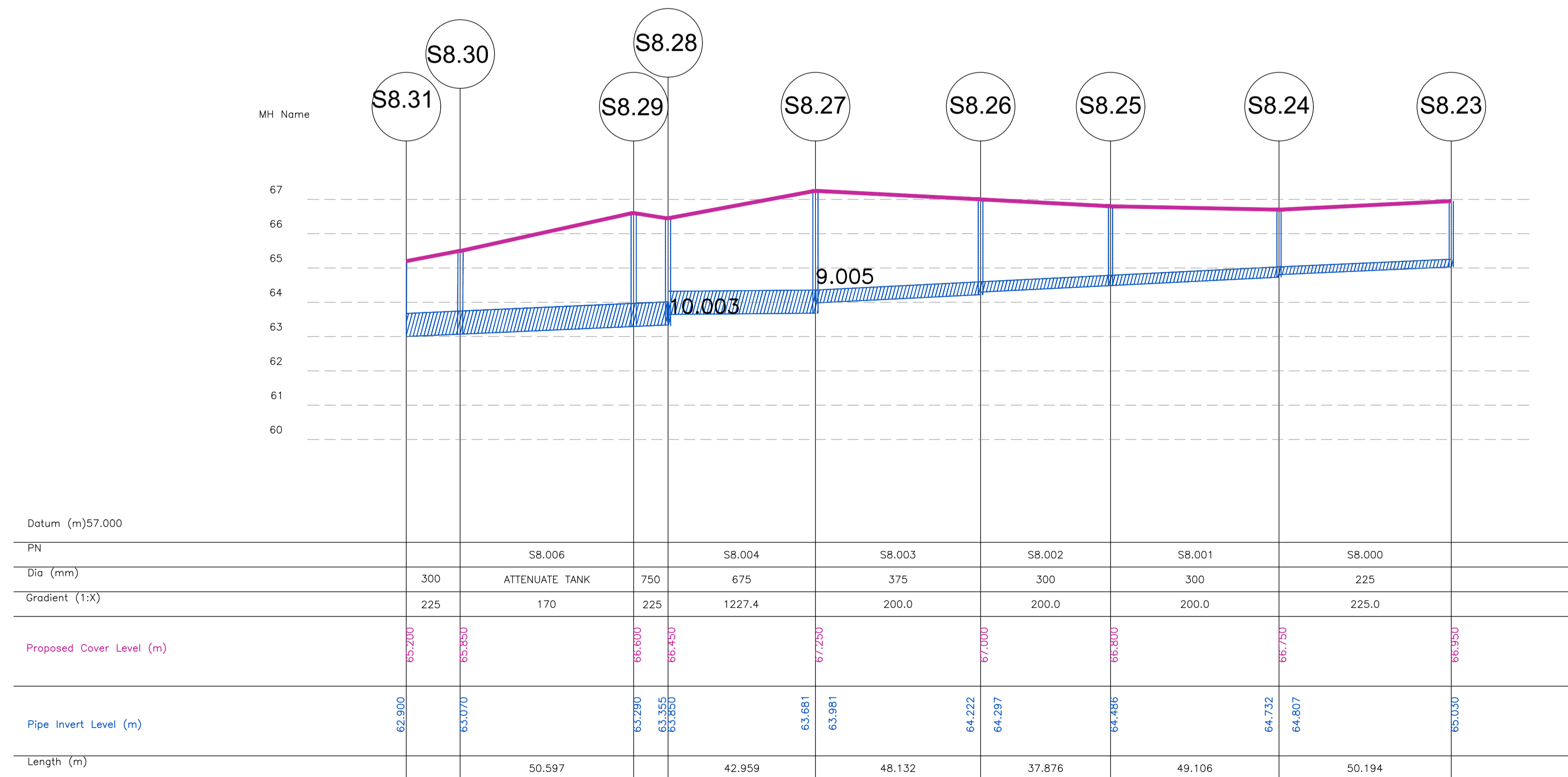
Surface Drains Section Scale - X 1:1000; Y 1:100
